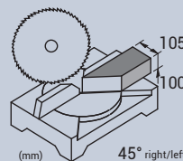
Corte 0°/45°: 100x105 mm
