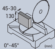
Corte rect: 130x45-30 mm
